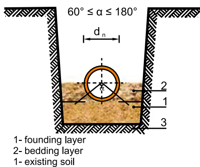
Figure 6.2 An example for laying in resistant soil
