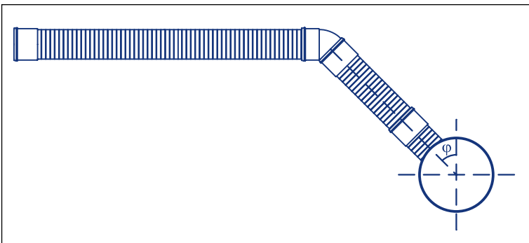
Figure 7.2 Joining of side sewer to a collector in case of displacement
