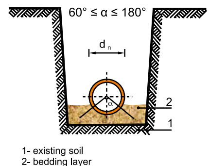
Figure 6.1 Laying in natural conditions
