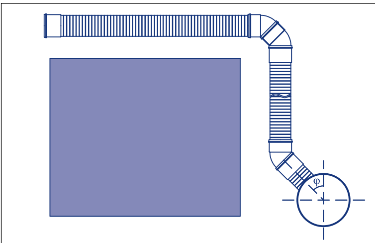
Figure 7.3 Joining of side sewer to a collector in case of displacement and an obstacle
