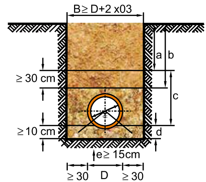
Figure 6.5 Pipeline section
