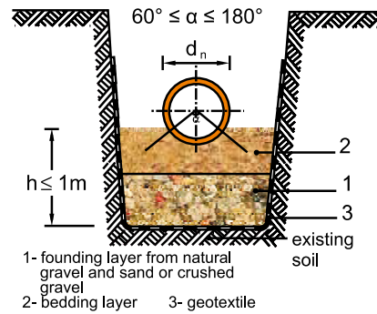
Figure 6.3 An example for laying in weak soil (loess) depth \leq 1.0 m
