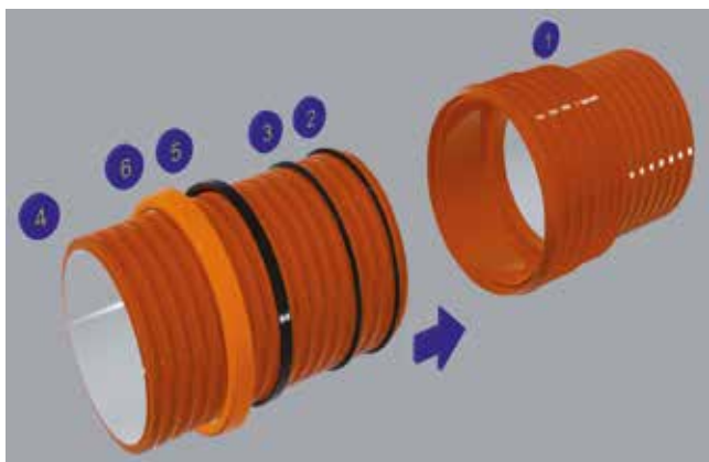
Figure 7.5 Pipes Ready For Assembly
