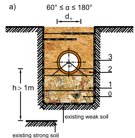
Figure 6.4 An example for laying in weak soil (loess) > 1.0 m
