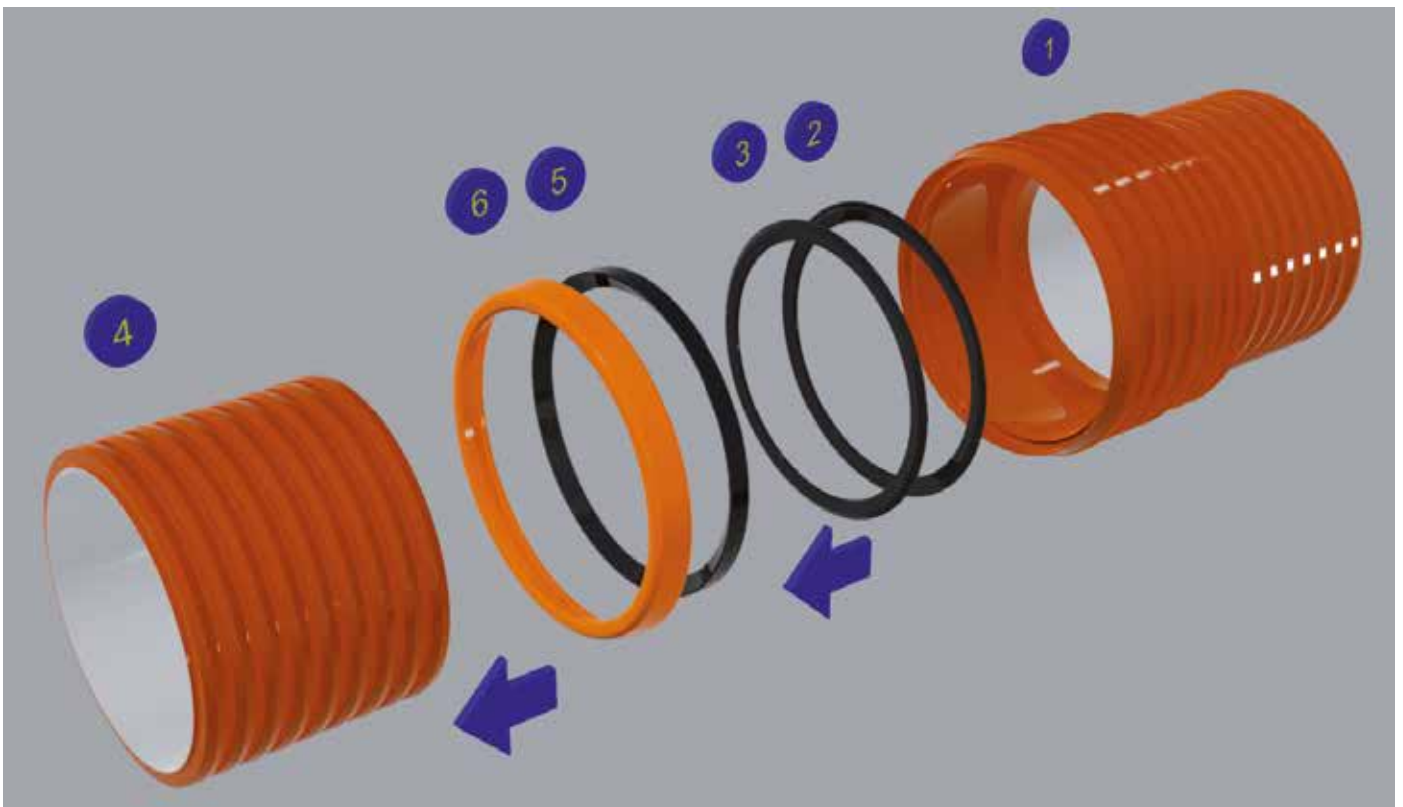
Figure 7.4 Necessary Elements For The Locked Socket Connection
