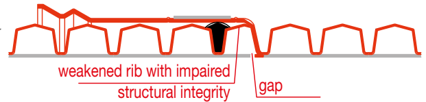
wrong coupling, due to wrong cutting
