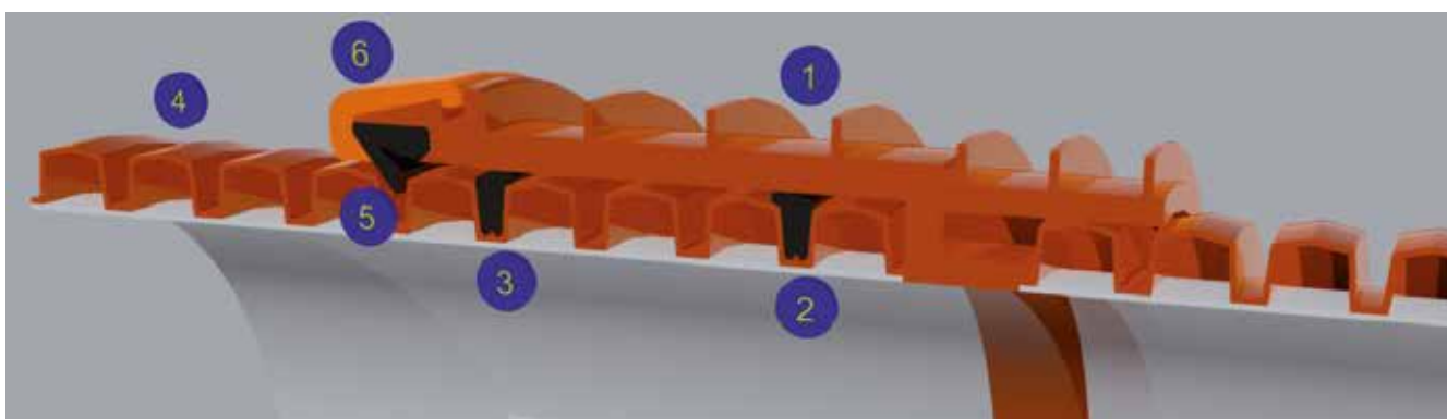
Figure 7.7 Pragma Locked Socket Connection – Detailed View
