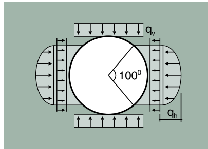
Figure 10.3 Scandinavian Model of soil pressure distribution
