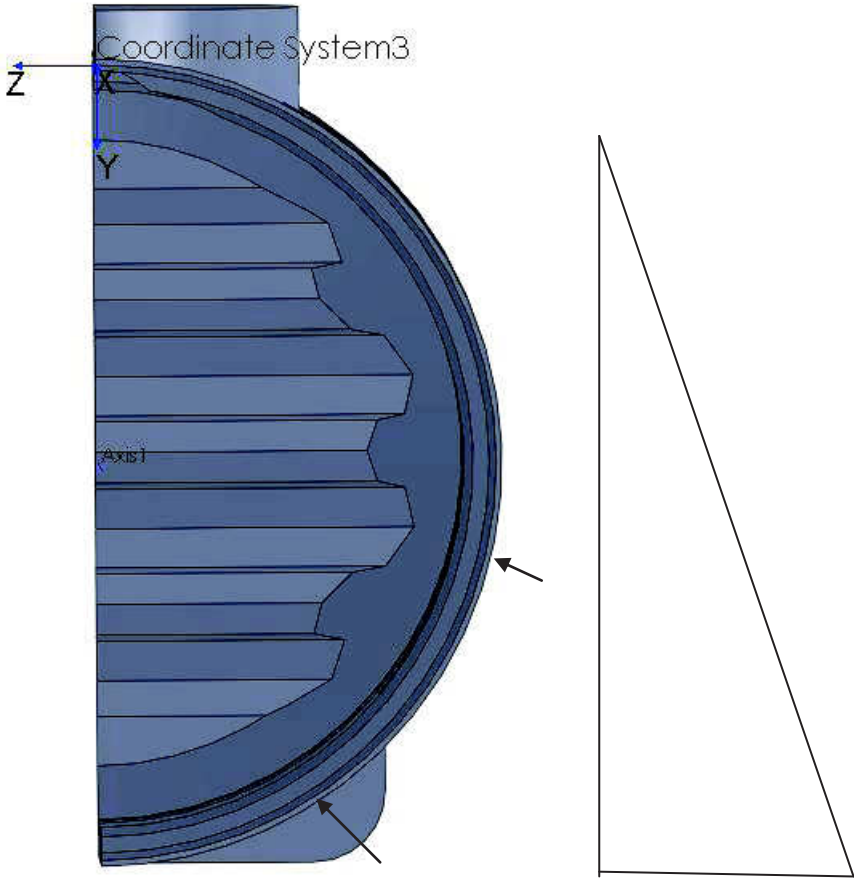
Figure 5: Hydrostatic load
