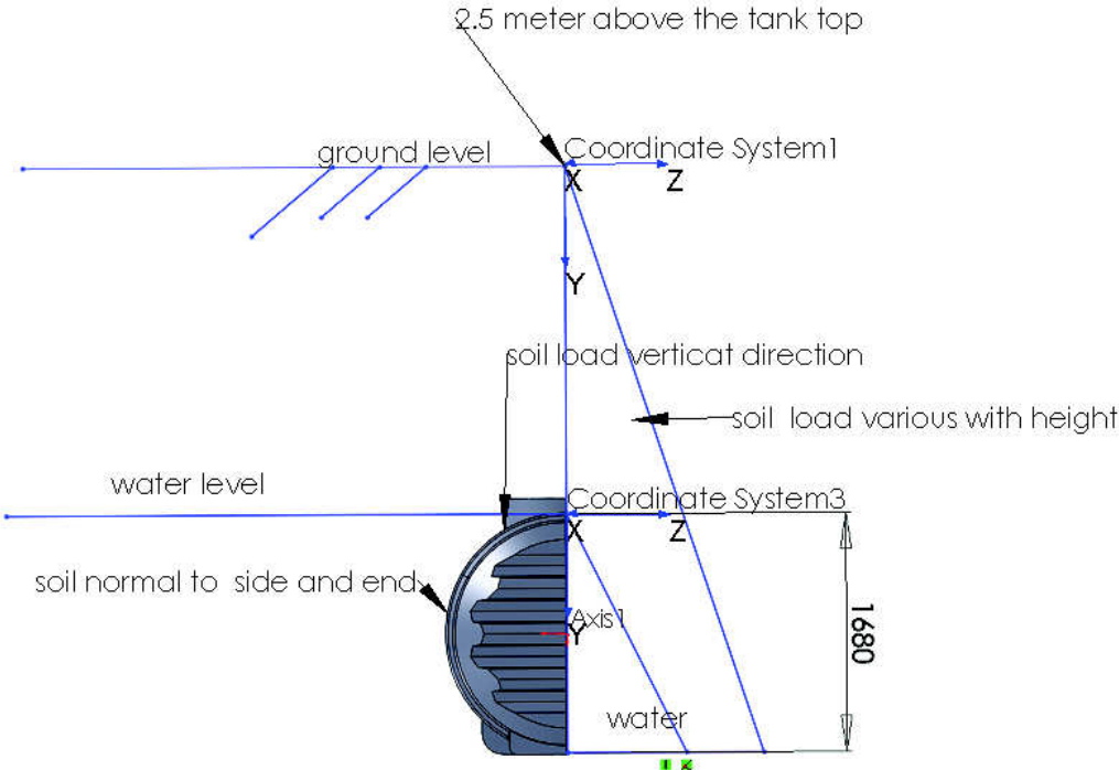
Figure 3: Loads
